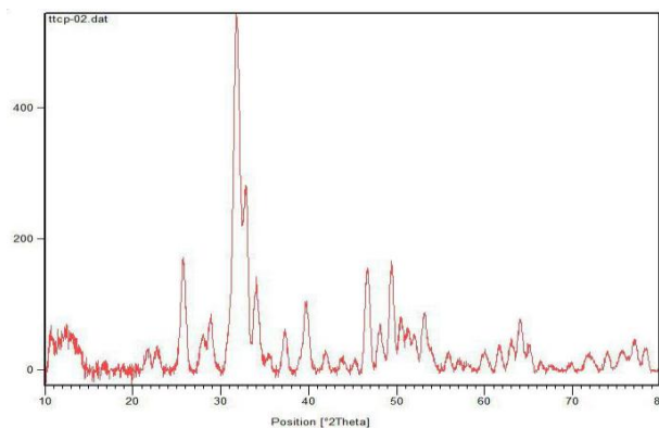
Figure 1. XRD spectrum of APA-TTCP
